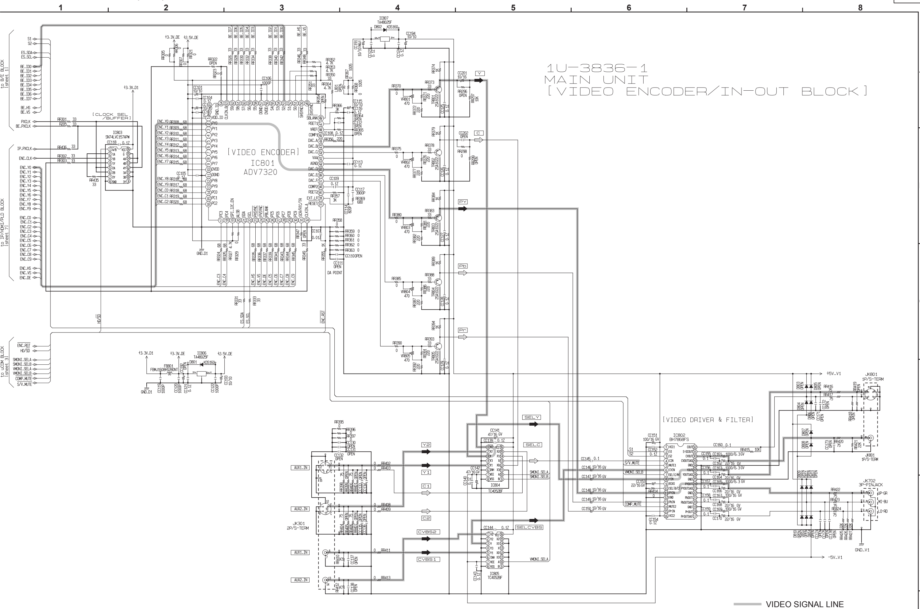
SCHEMATIC DIAGRAMS (9/17) 1U-3836-1 MAIN UNIT(8/8) VIDEO ENCODER / IN-OUT BLOCK
