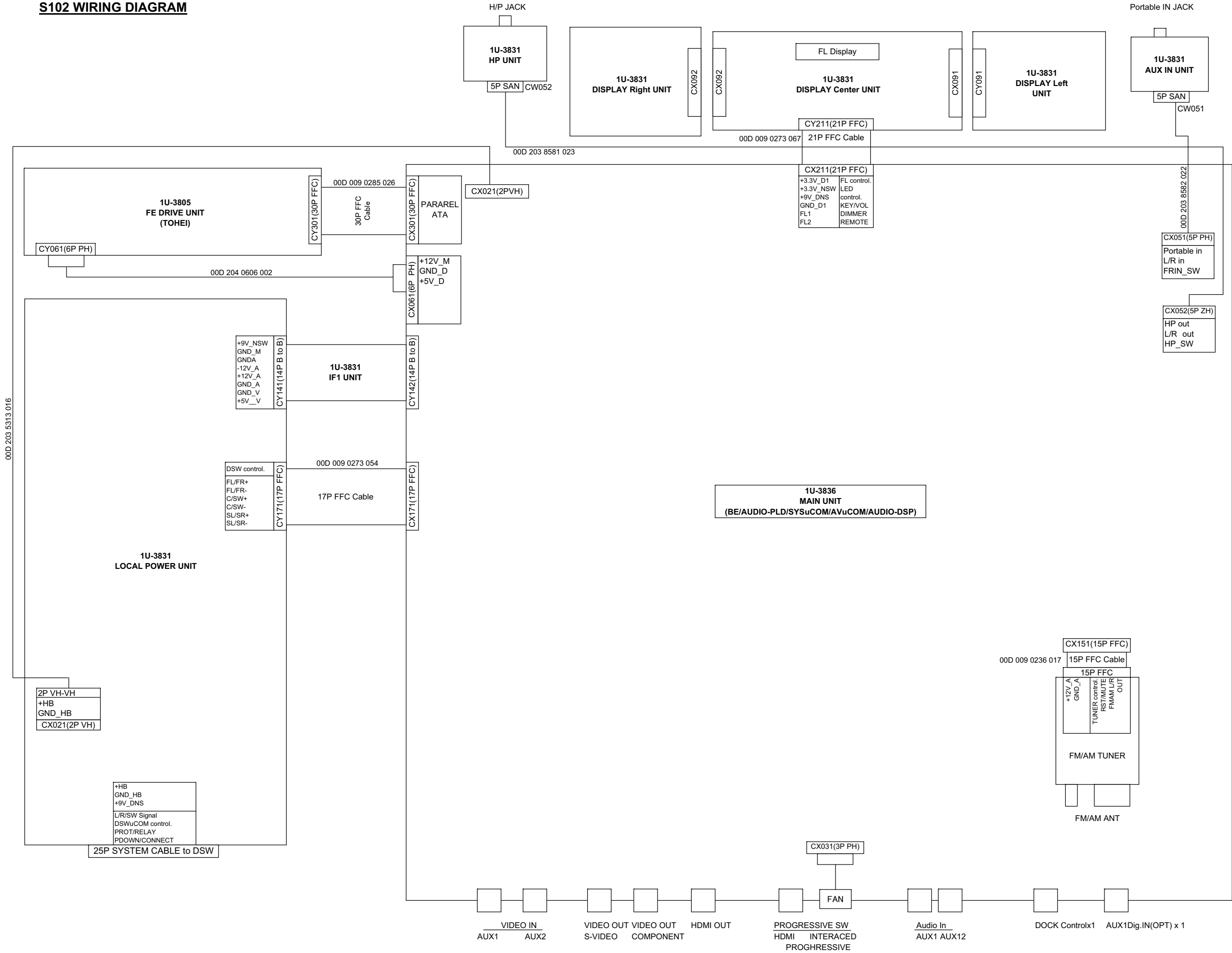
S102 WIRING DIAGRAM
