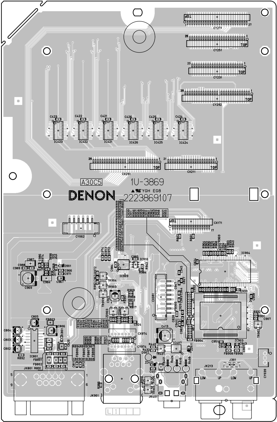
COMPONENT SIDE
