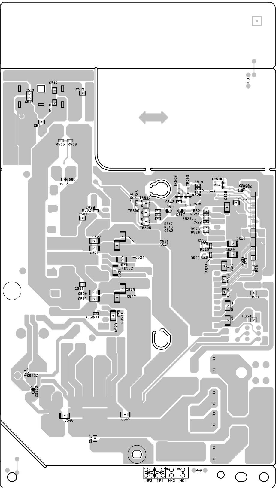
FOIL SIDE
