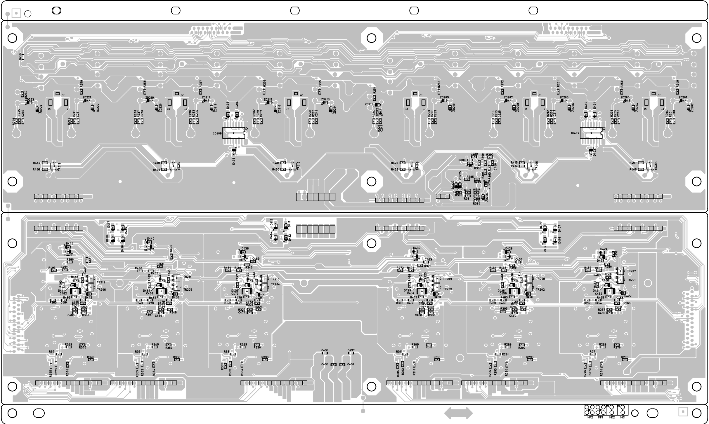
FOIL SIDE
