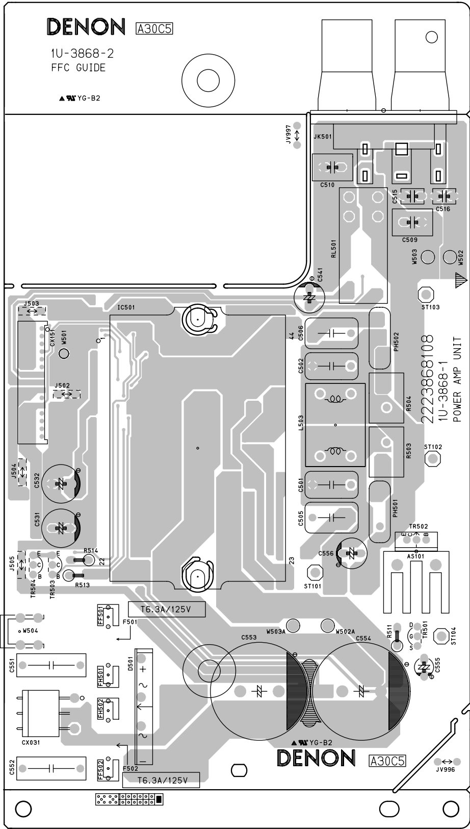
COMPONENT SIDE
