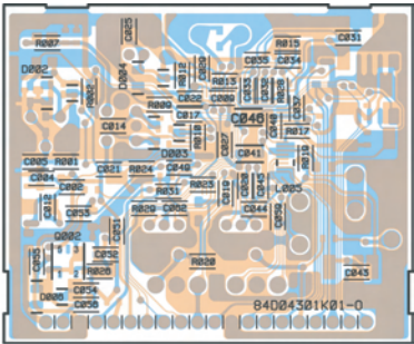
RADIO P.W.Board (Foil Side View)
