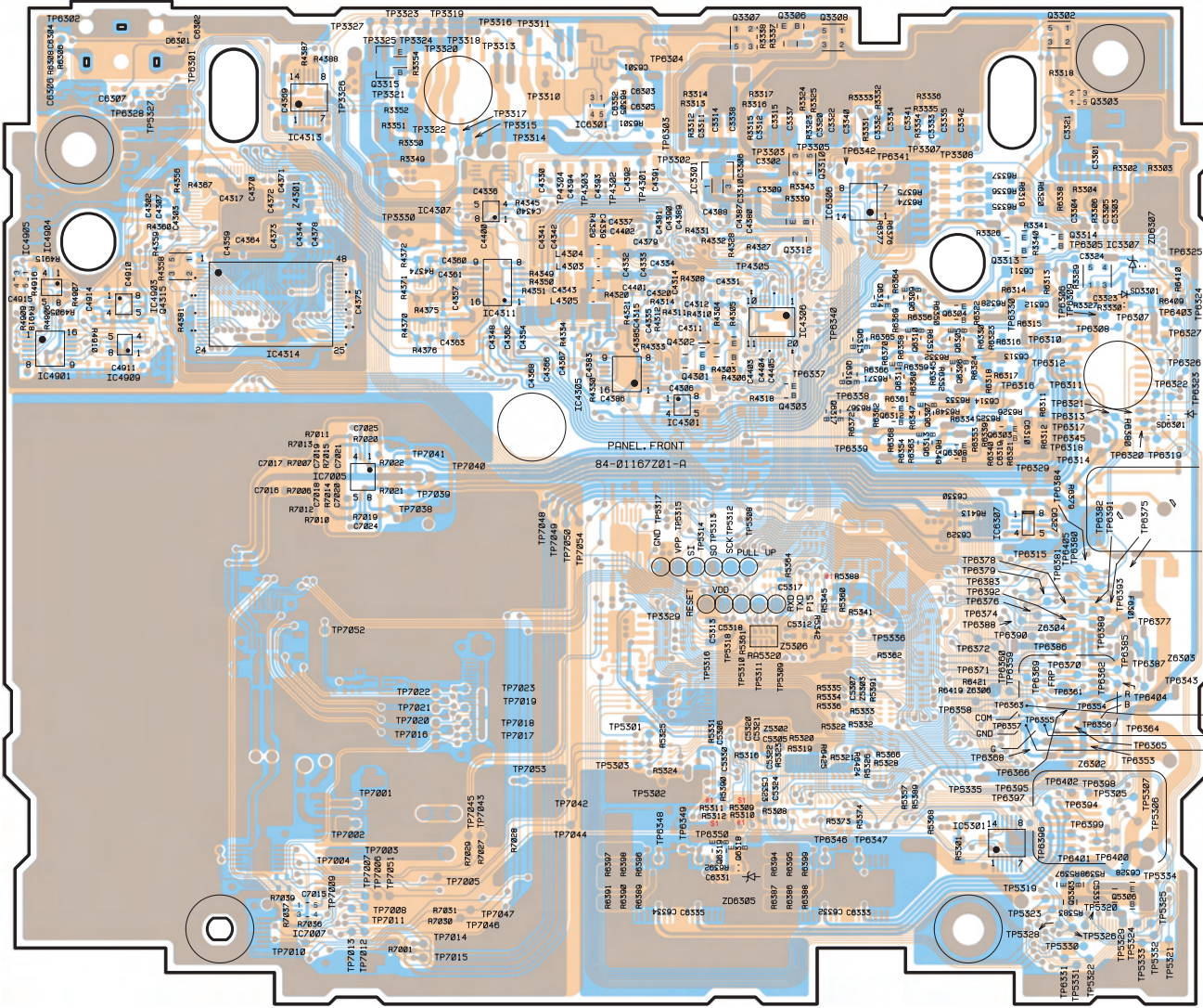
FRONT P.W.Board (Foil Side View)
