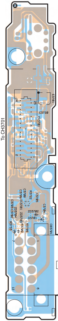
POWER P.W.Board (Component Side View)
