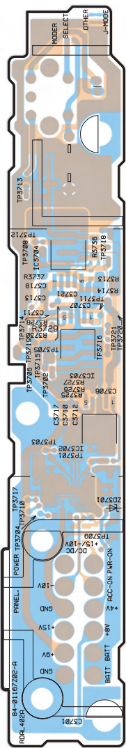
POWER P.W.Board (Foil Side View)
