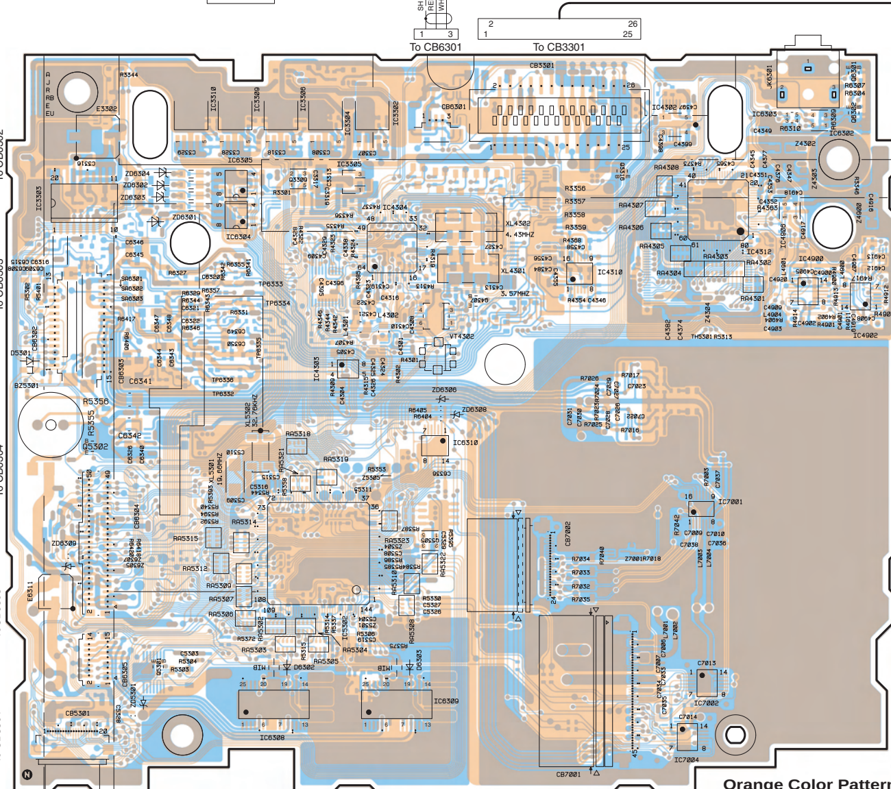
FRONT P.W.Board (Component Side View)
