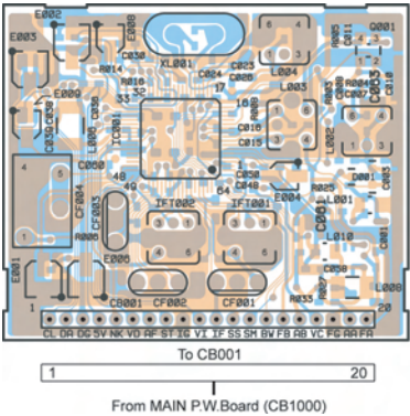
RADIO P.W.Board (Component Side View)
