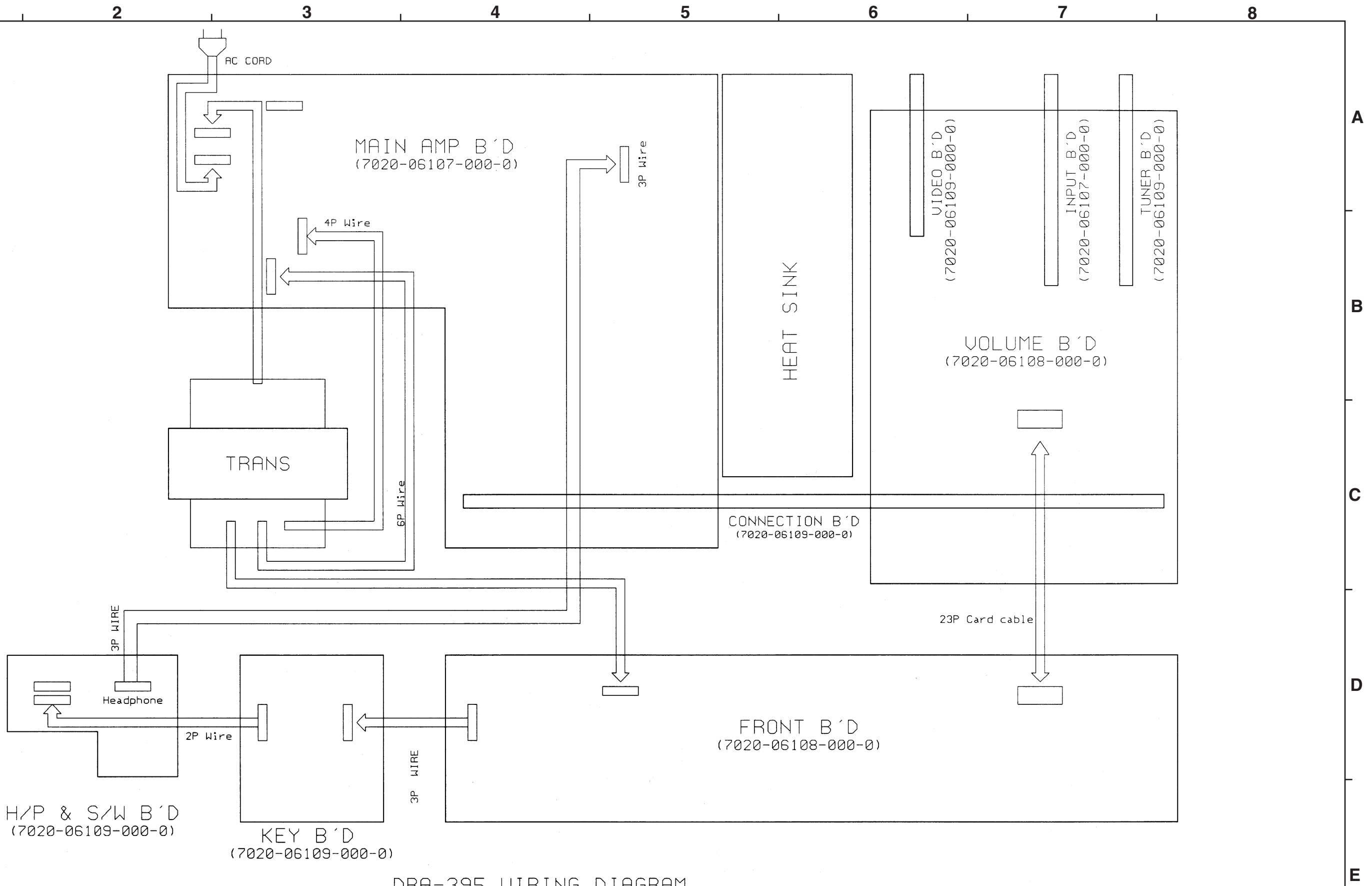
DRA-395 WIRING DIAGRAM
