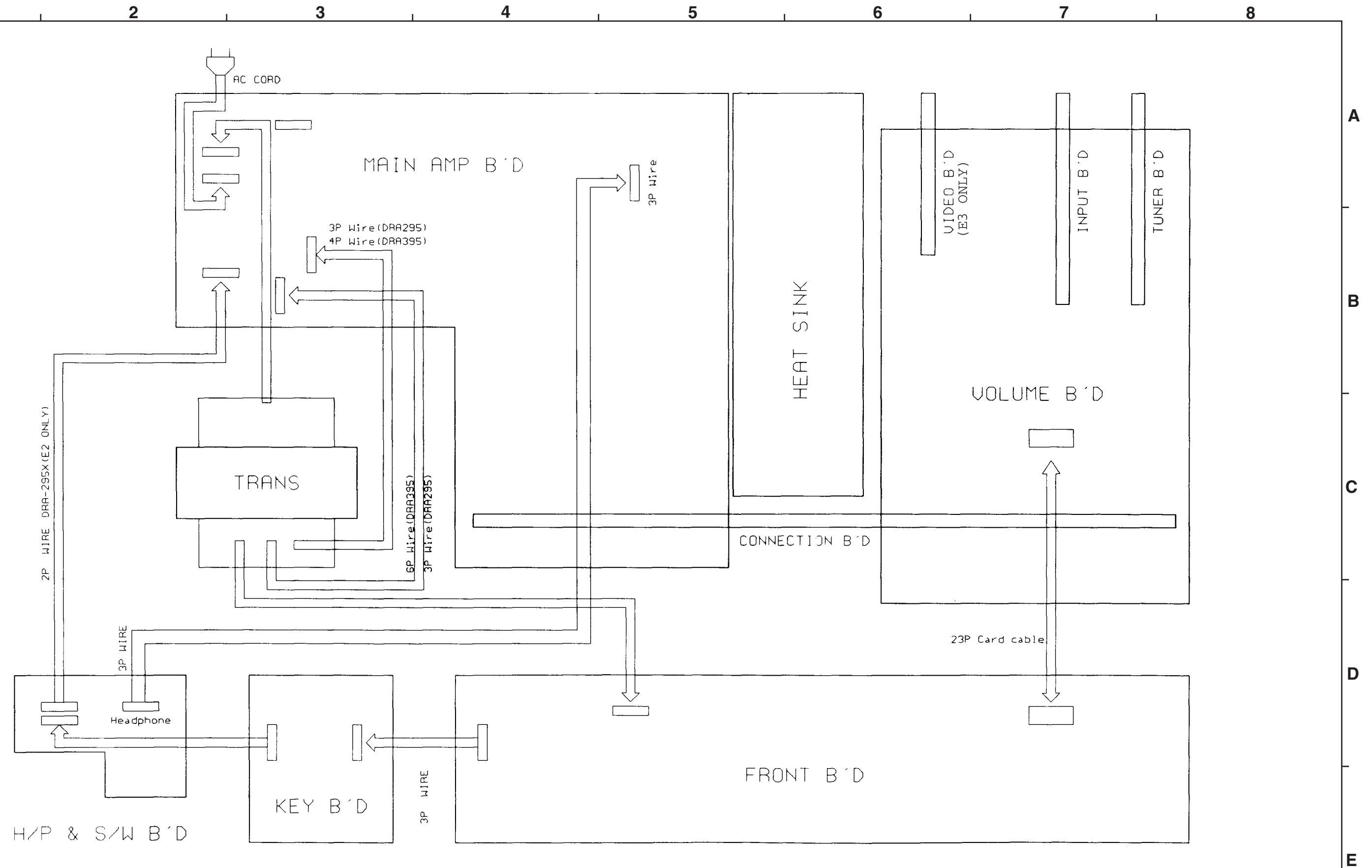
DRA-295 WIRING DIAGRAM
