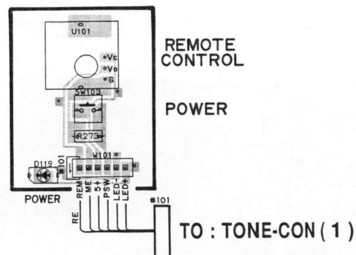
MAIN P. C. B. ( 3 )
