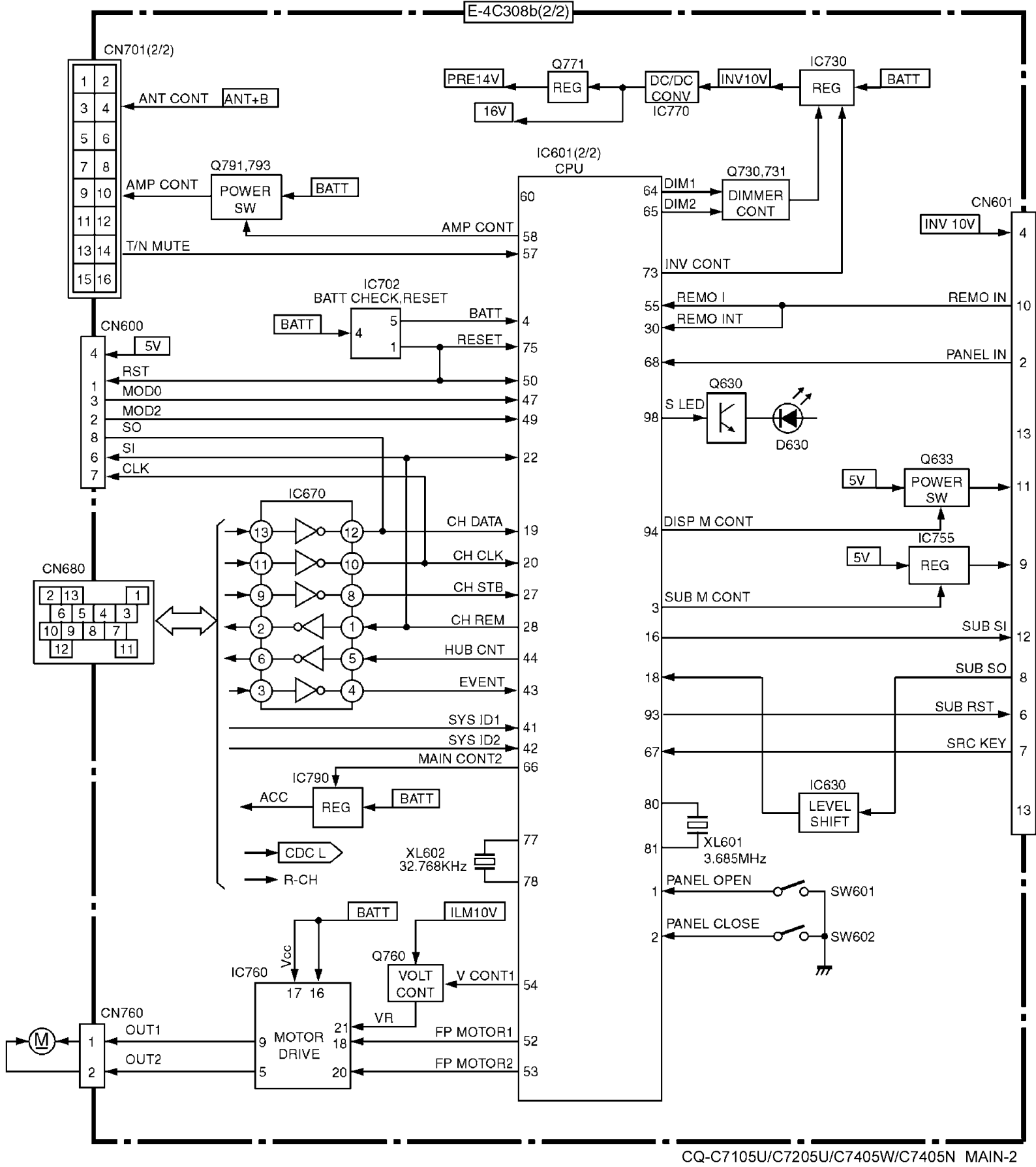
CQ-C7105U/C7205U/C7405W/C7405N MAIN-2
