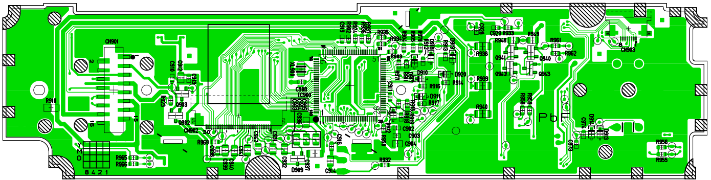
[E-4C310][BOTTOM VIEW]
