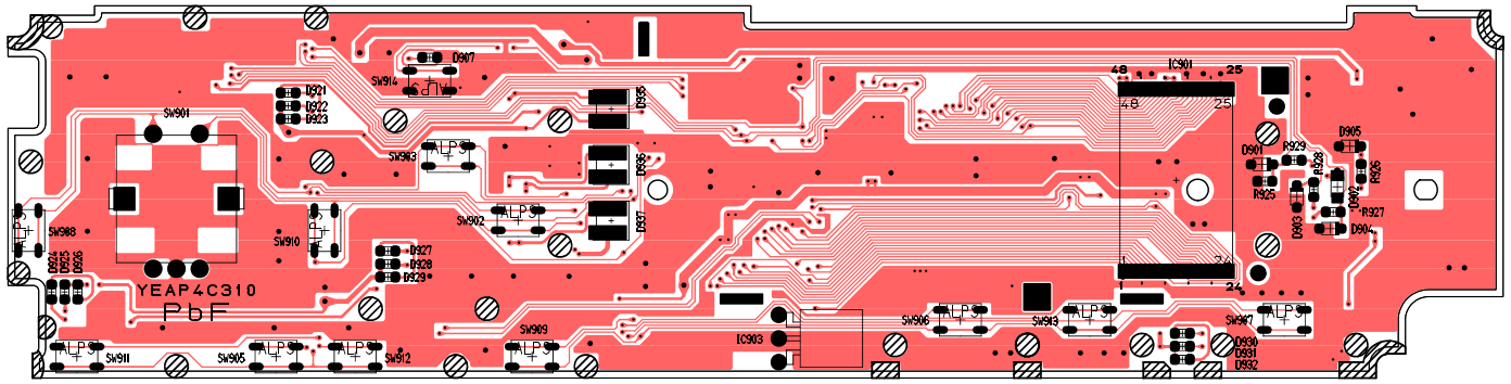
[E-4C310][TOP VIEW]
