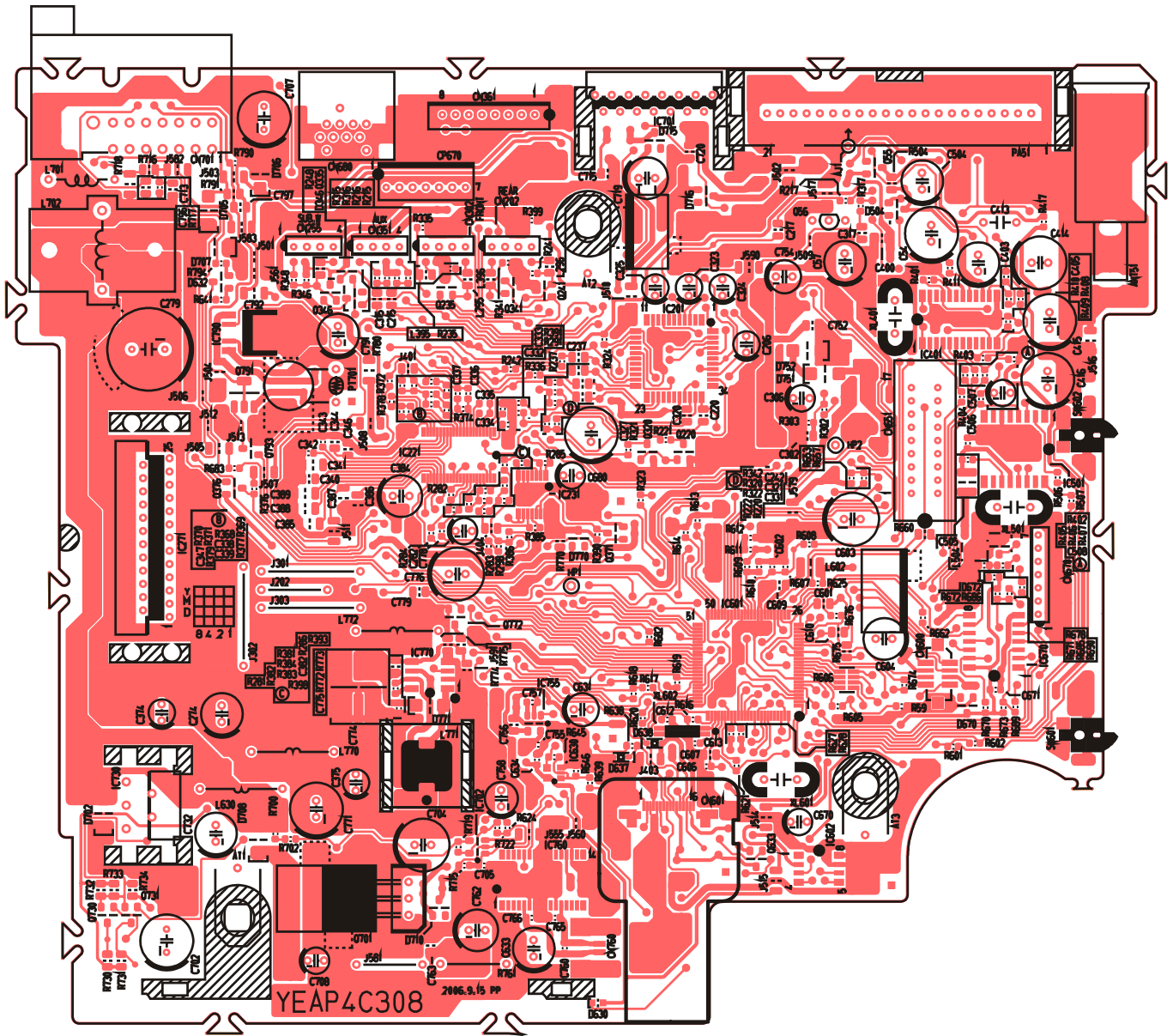
[E-4C308a][TOP VIEW]
