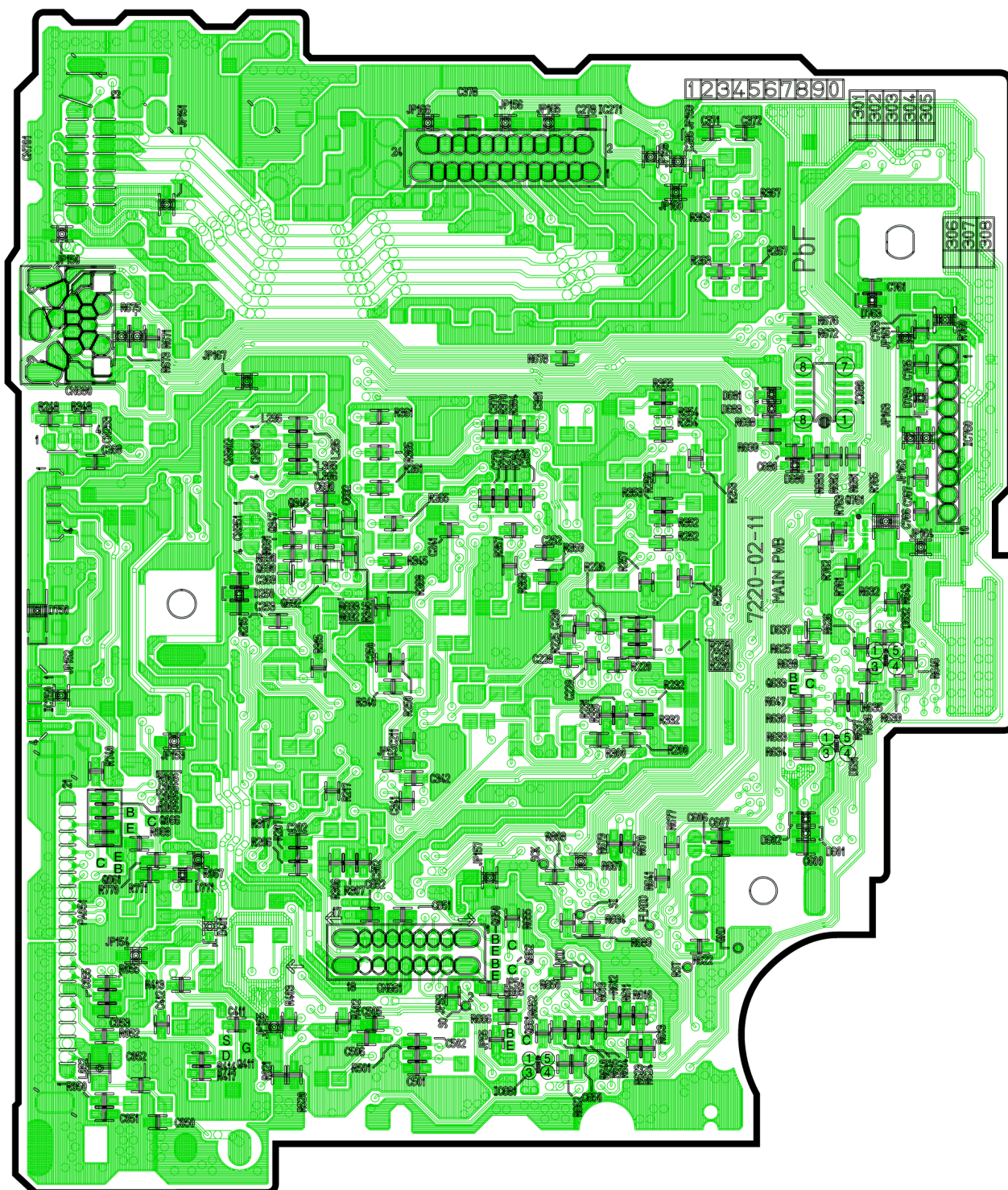
[7220-02-11] [Bottom View]
