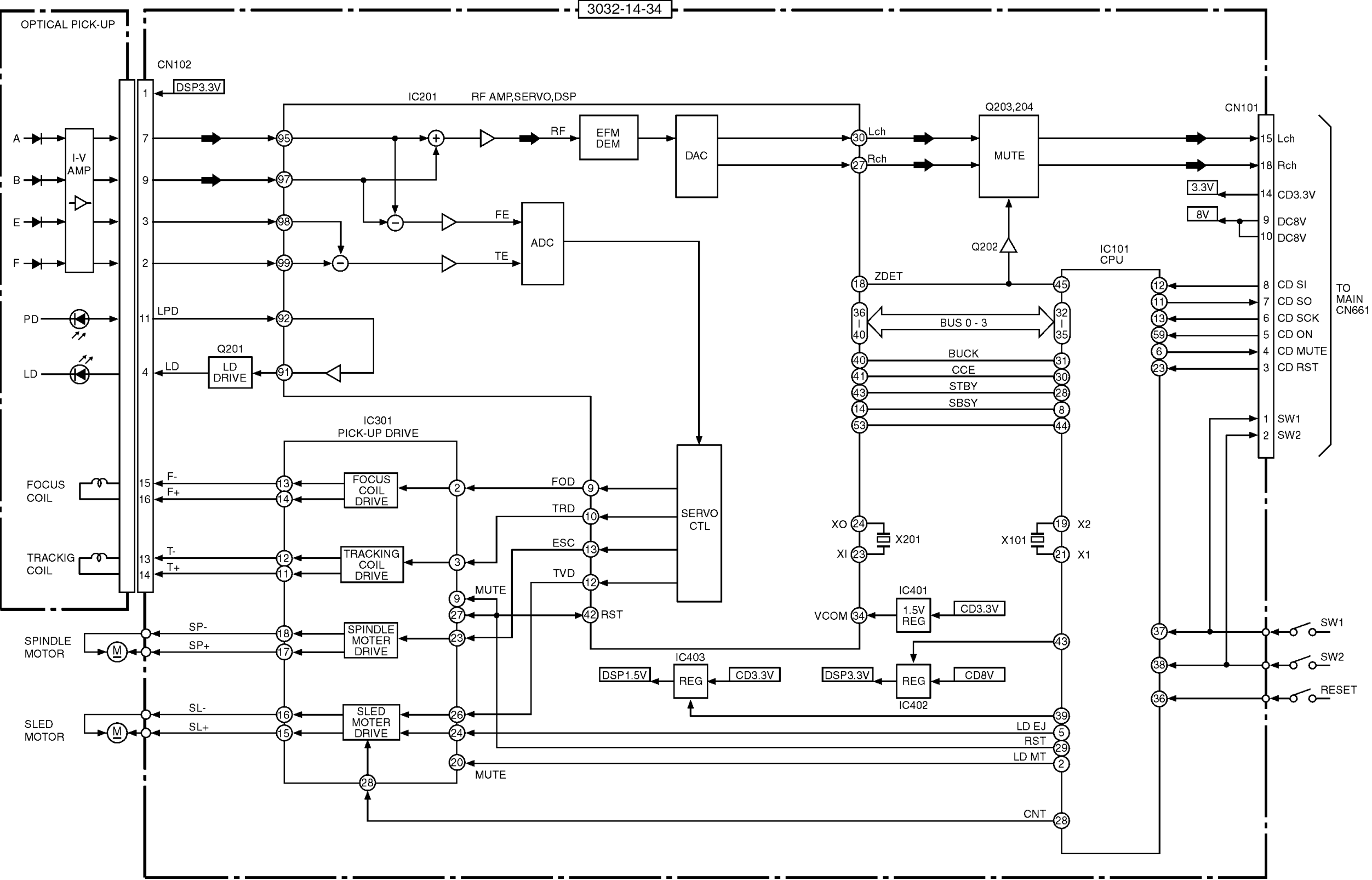
CQ-C5403U/C5303U CD Deck Block Printed in Japan 2005.11 (K) (Recycled Paper)
