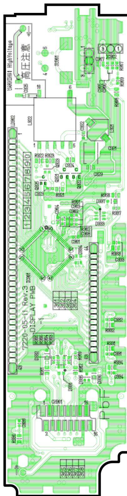
[7220-05-11] [Votpm View]
