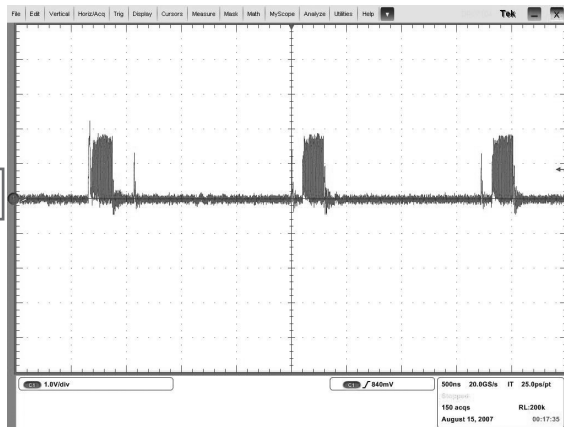
MT8520 DDR2_A_BA[0]
