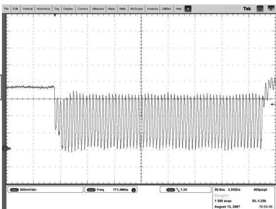
MT8520 DDR2_A_CAS#
